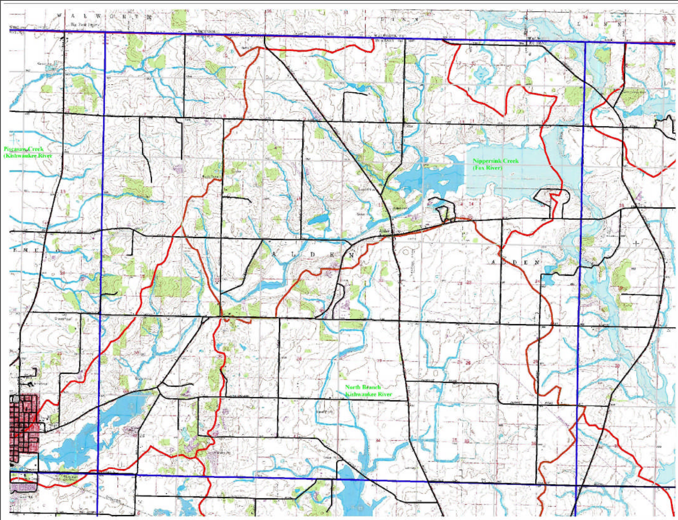
Alden Township Hydrologic Atlas (Flood of Record) and Watershed Boundaries
