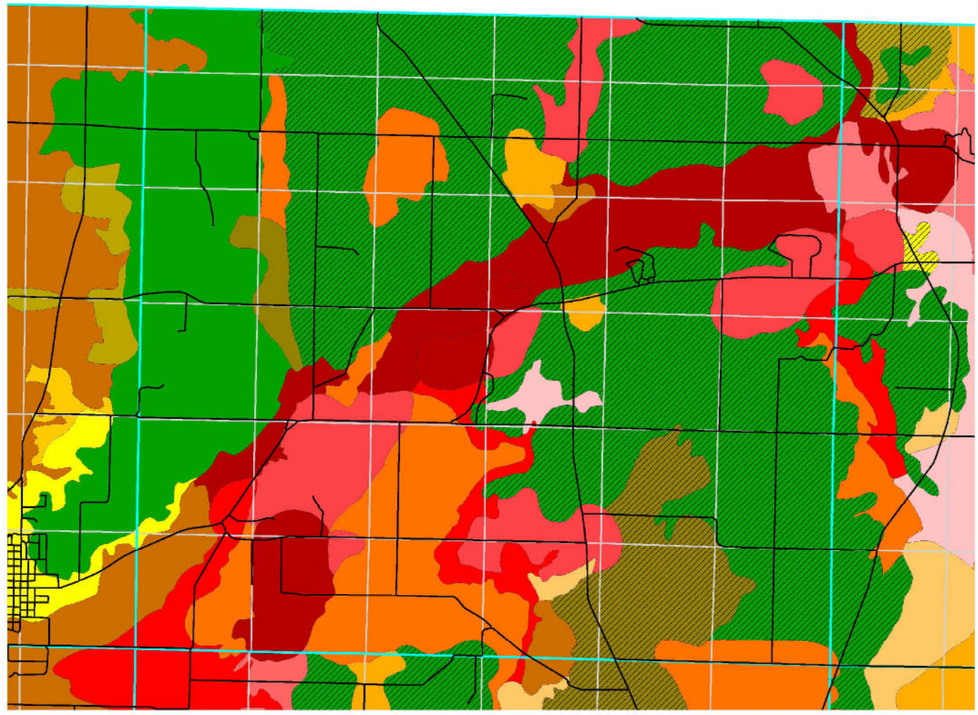
Alden Township Aquifer Sensitivity to Septic System Contamination
